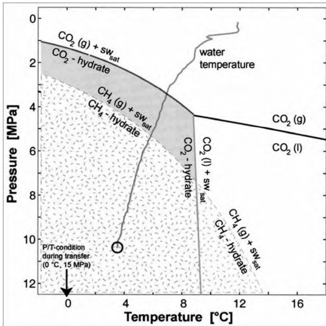
(Ignore the notation "P/T-condition during transfer (0 °C, 15 MPa)"; the diagram is from another document that is concerned with CO 2 hydrate as well) Slide 6. Methane-hydrate stability diagram. Please ignore the CO 2 hydrate curves.
