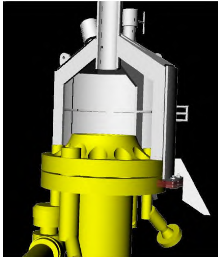
Slide 5a. The TopHat4 as conceived, mounted on the seafloor structure (yellow). The block rubber gasket is shown in red.
